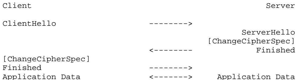
Figure 2. Message flow for an abbreviated handshake
